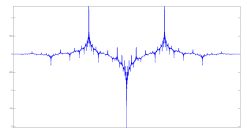
Figure 3 : CDF 9-7 wavelet
