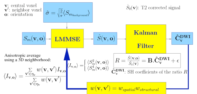
Figure 1: The Rician noise correction algorithm.
